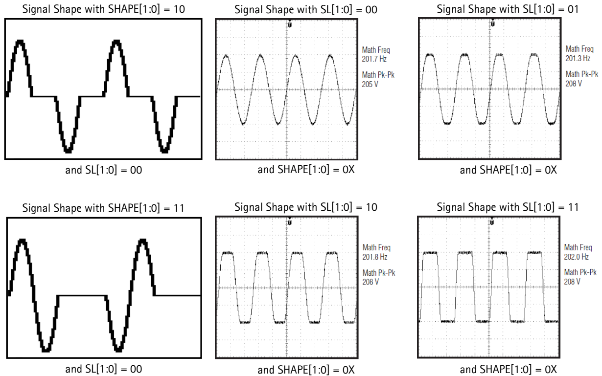
Figure 4: Signal shapes
